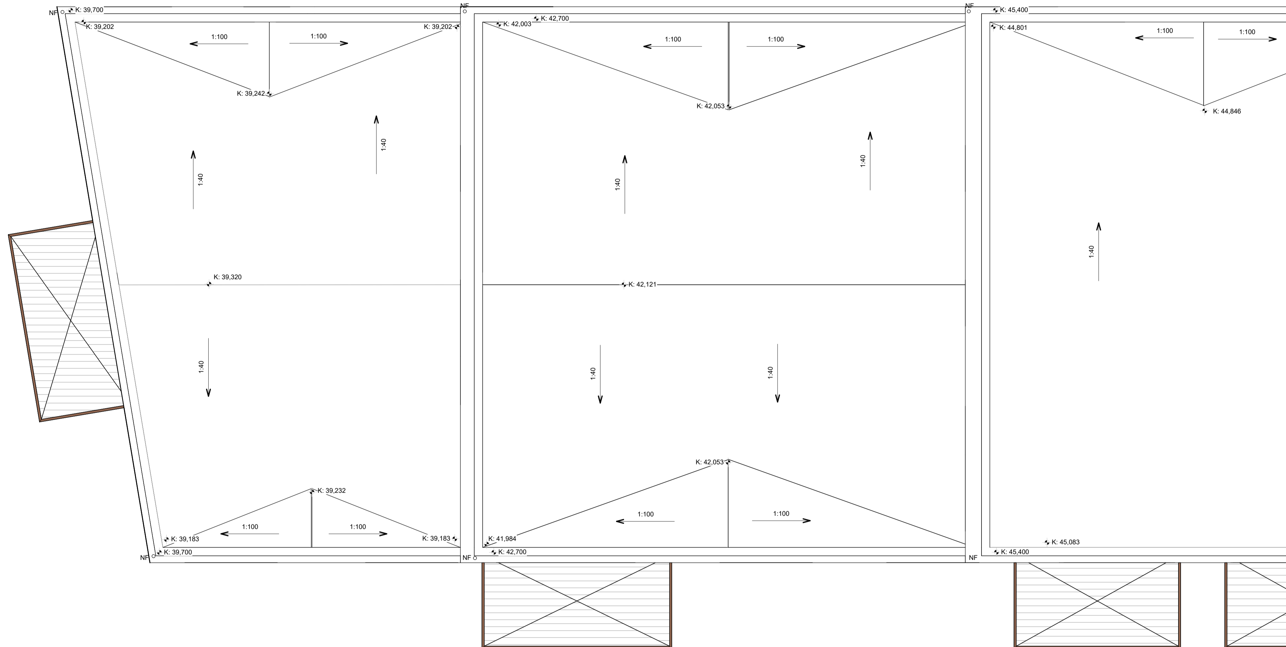
Þakhallaplan - Mhl. 02 - 1/2 1:50
